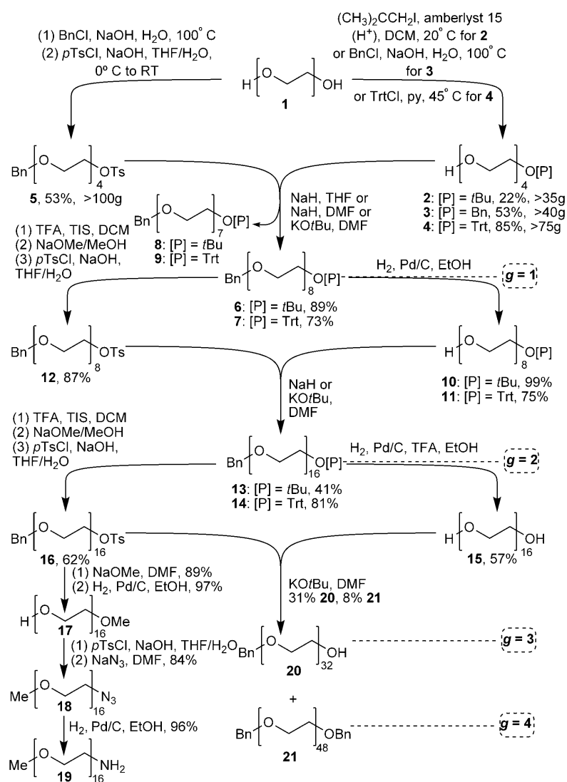
Scheme 1. PEG Syntheses: Chain doubling mode C synthesis of highly pure PEG oligomers. Trt = trityl, pTs = para -toluenesulfonyl, TIS = triisopropylsilane, DCM = dichloromethane, TFA = trifluoroacetic acid, [P] = protecting group.
